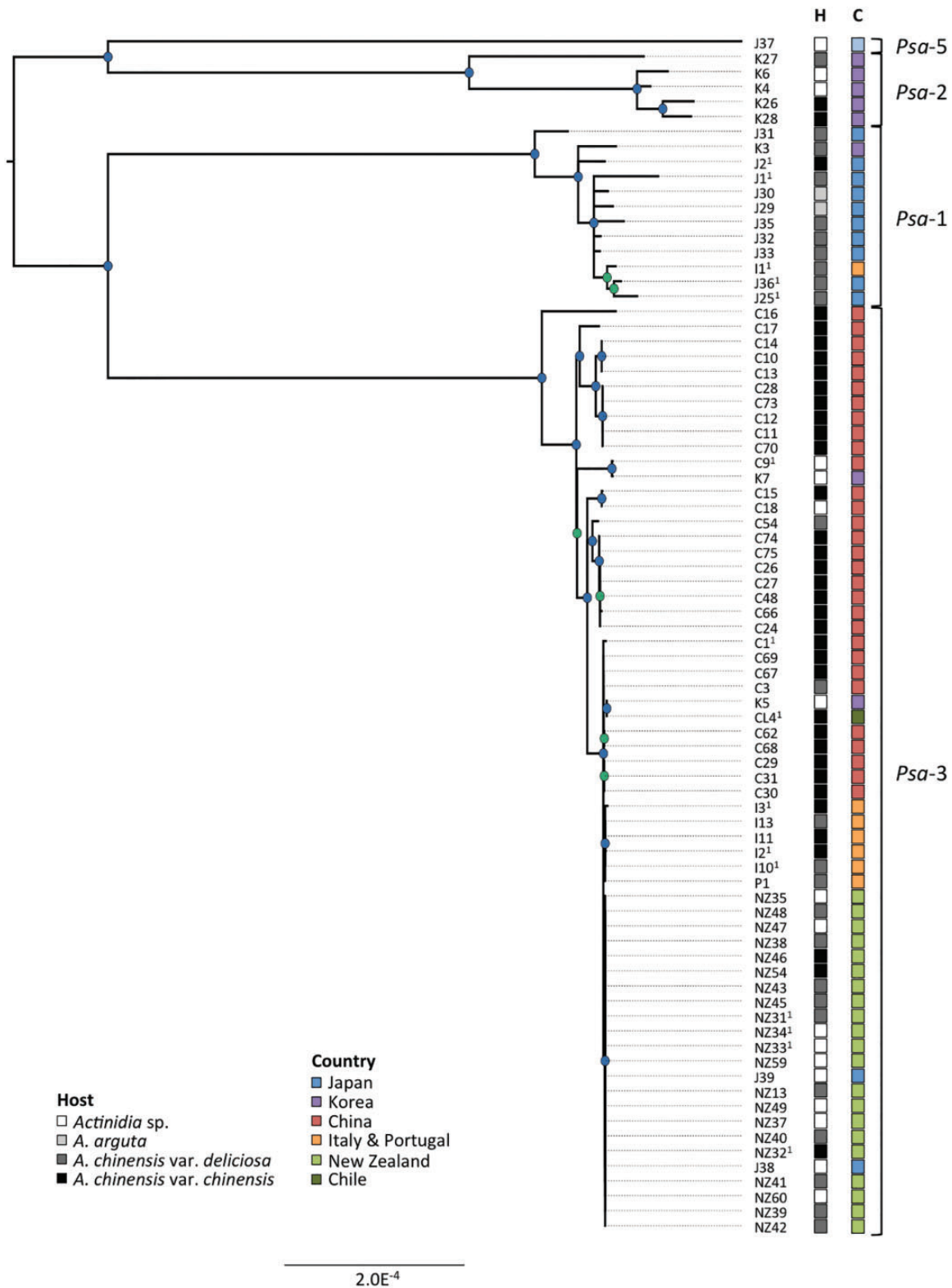
Fig. 1. —Phylogeny of Psa . RaxML Maximum likelihood tree based on 1,059,722bp nonrecombinant core genome alignment including 2,953 variant sites. FigTree was used for phylogeny visualization. All nodes displayed have bootstrap support values above 50% (50–75% in green, 76–100% in blue). Host (H) and country (C) of isolation is displayed in the first and second column, respectively. Clade designations are shown at right.
