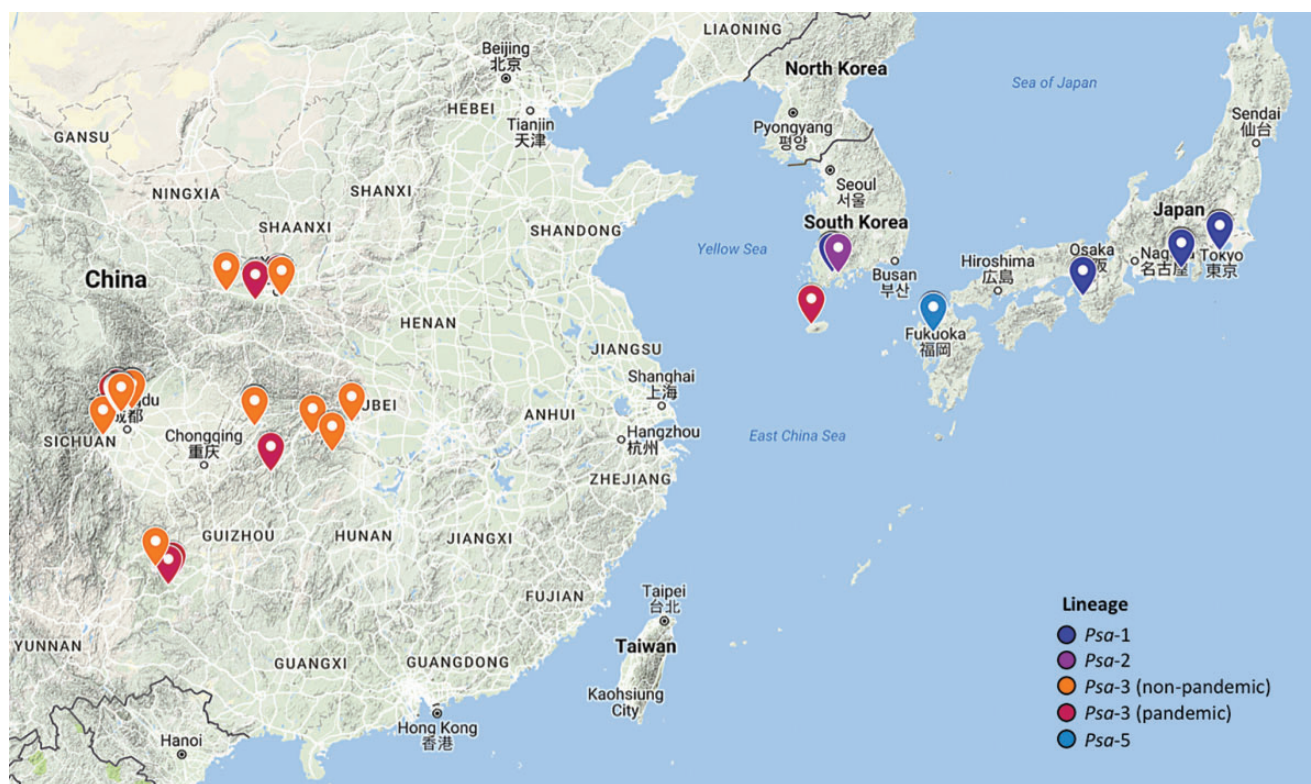
FIG. 3. — Psa isolation locations in East Asia. Markers correspond to location of isolation. Color corresponds to the isolate membership in each clade according to the phylogeny displayed in fig. 1. Only isolates for which the specific location of isolation is known are displayed here.
