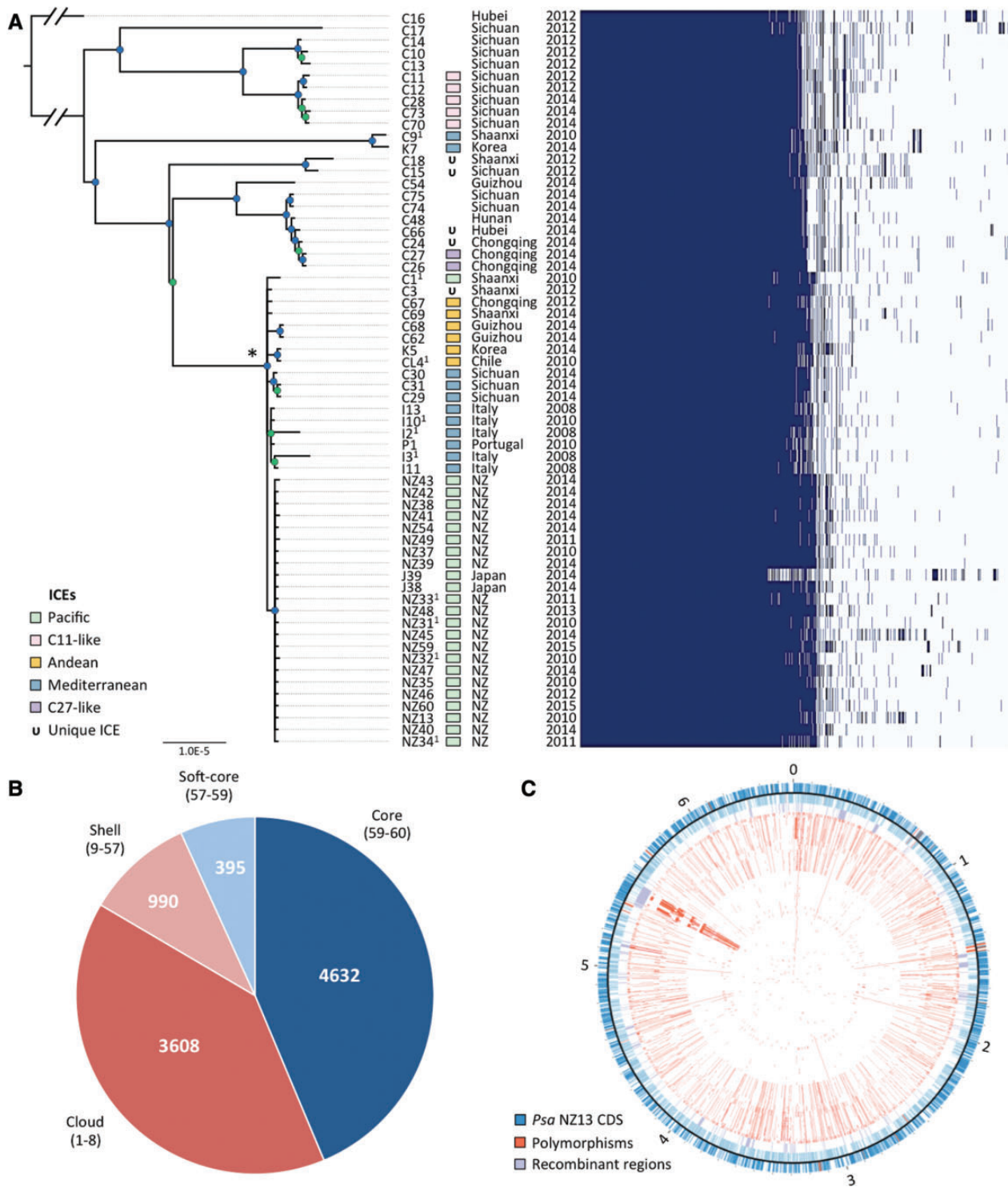
Fig. 2. —Phylogeny of Psa -3. (A) RaxML Maximum likelihood tree based on 4,853,155bp nonrecombinant core genome alignment including 1,948 variant sites. FigTree was used for phylogeny visualization. All nodes displayed have bootstrap support values above 55% (55–80% in green, 81–100% in blue). The asterisk denotes the pandemic lineage. Integrative and conjugative element (ICE) presence; province (China) or country and year of isolation shown at right, followed by presence/absence matrix of all core and accessory genes. (B) The core and flexible genome of Psa -3. Parenthetical numbers represent the number of strains in the core, soft-core, shell, and cloud genomes. (C) Polymorphisms and recombinant regions mapped onto Psa NZ13 reference genome using CIRCOS (Krzzywinski et al. 2009). Psa NZ13 CDS are displayed in the first and second ring (blue), with annotated Type 3 secretion system and effectors highlighted (red). Inner rings display polymorphisms in Psa -3 genomes ordered from most to least divergent relative to Psa NZ13. The most polymorphic region corresponds to the location of the integrative and conjugative element (ICE) in Psa NZ13.
